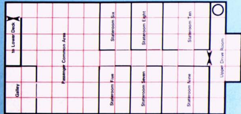
Free Trader Upper (Passenger) Deck
