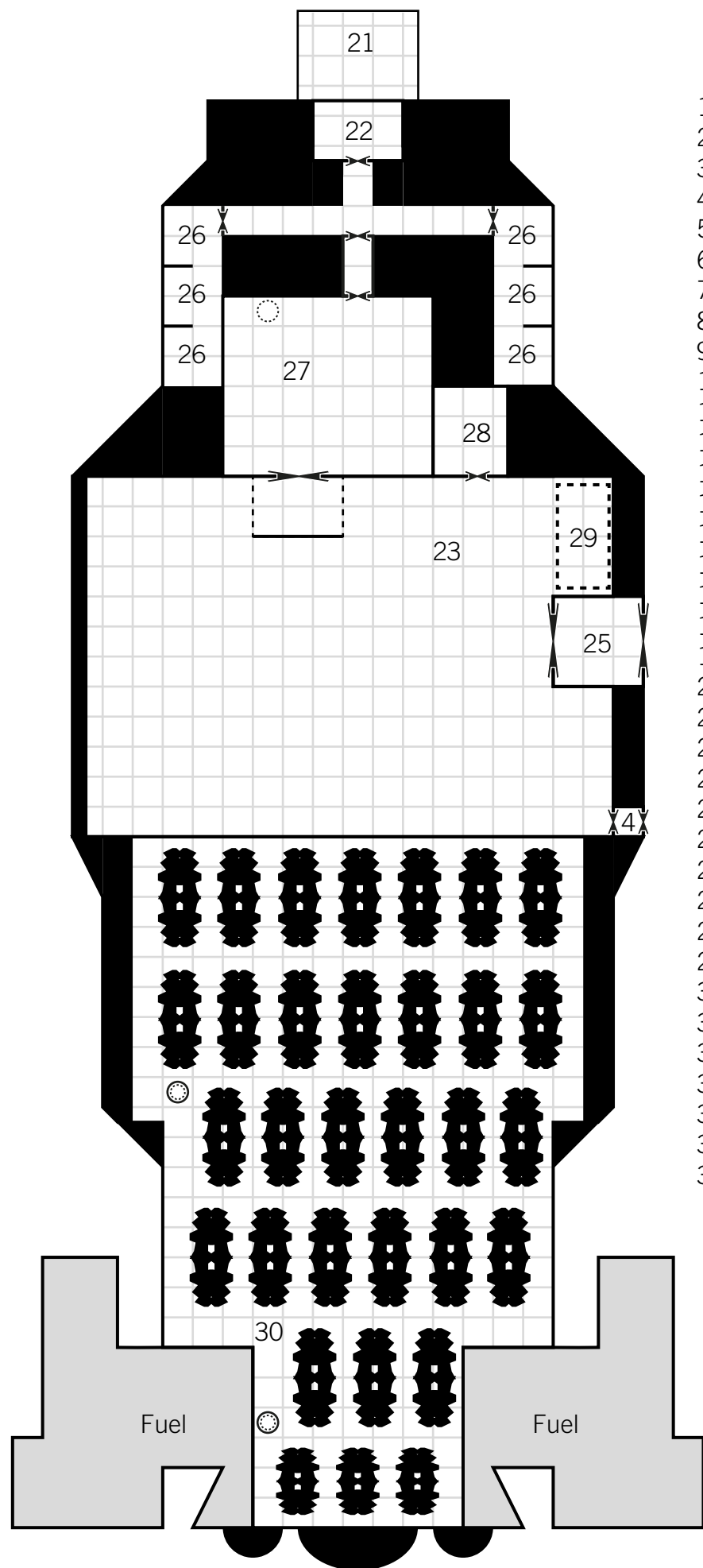
Deck E
